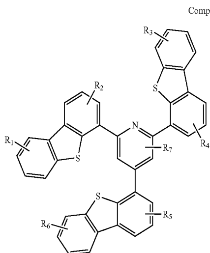
Compound 33G
