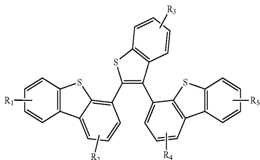
Compound 11G
