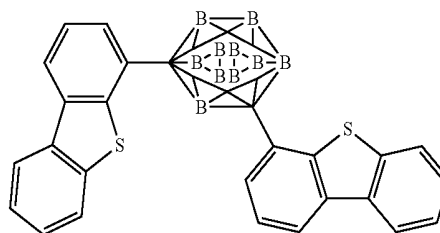
Compound 14
