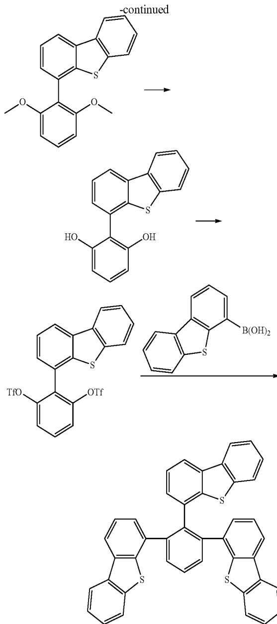
Compound 20
