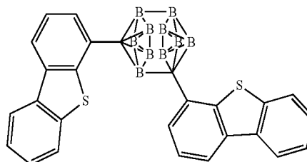
Compound 14
