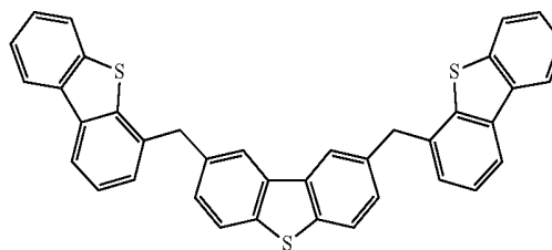
Compound 15
