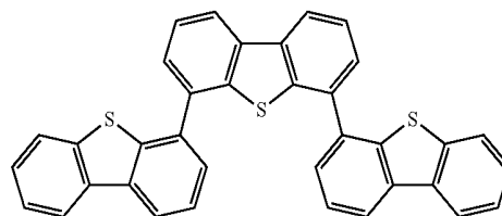
Compound 4
