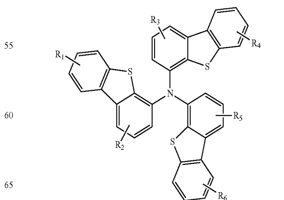
Compound 9G
