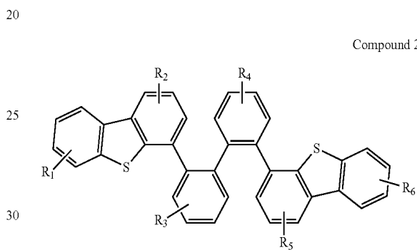
Compound 9
