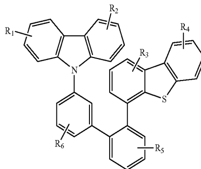
Compound 12G
