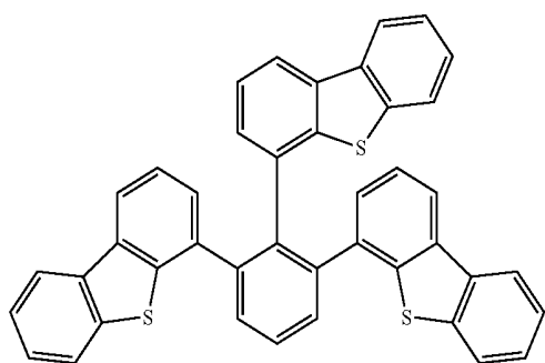
Compound 20
