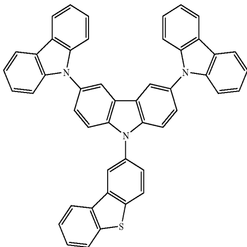
Compound 18
