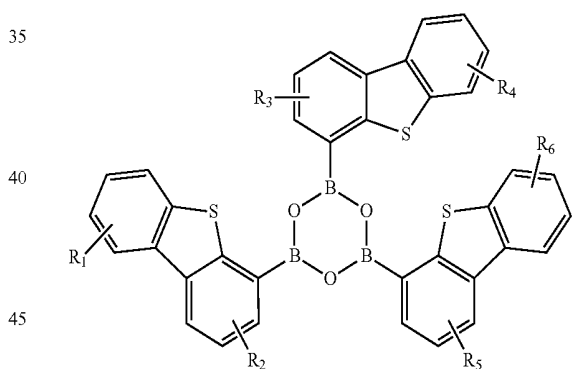
Compound 8G
