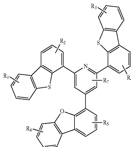
Compound 35G
