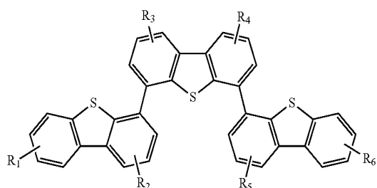
Compound 3G
