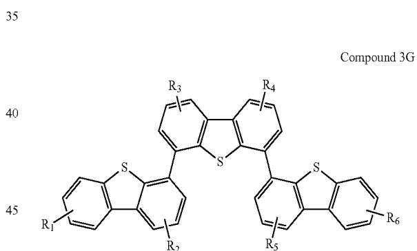
Compound 10
