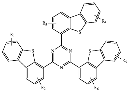
Compound 7G
