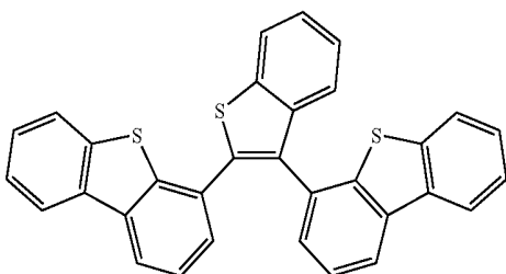
Compound 10
