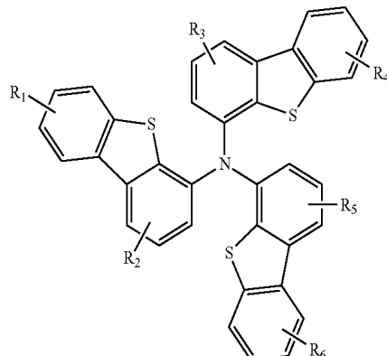
Compound 9G
