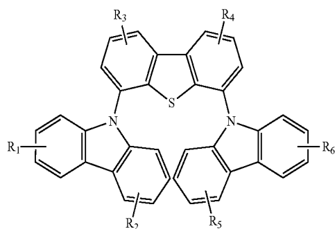
Compound 4G
