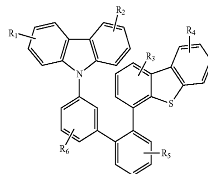
Compound 12G
