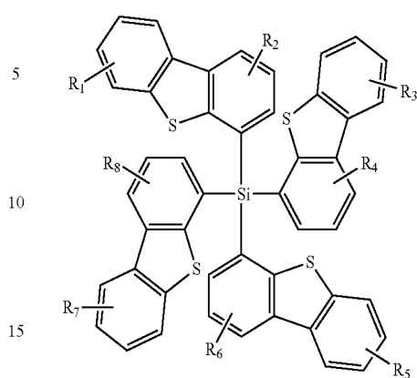
Compound 12G
