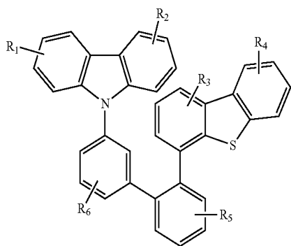
Compound 12G
