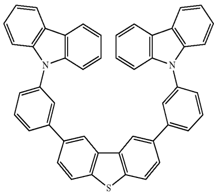
Compound 18
