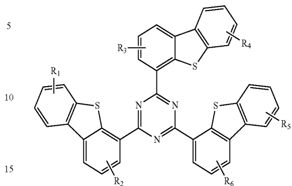
Compound 7G
