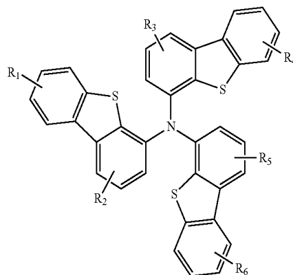
Compound 9G
