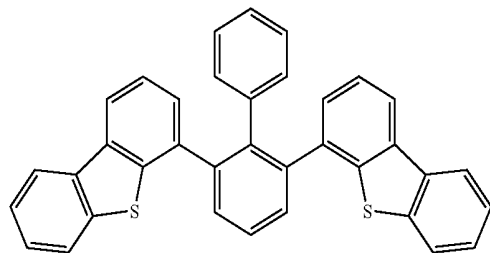
Compound 22
