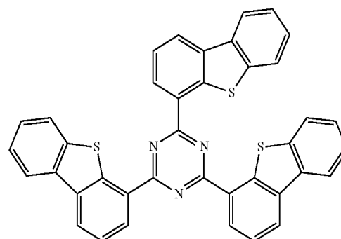
Compound 6
