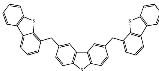
Compound 15
