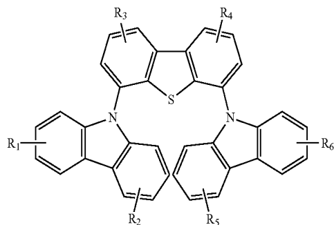
Compound 4G
