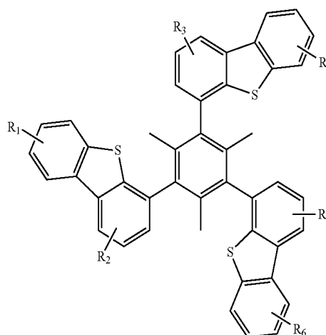
Compound 5G
