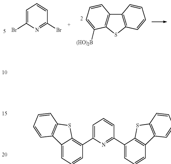
Compound 23
