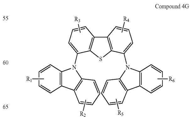
Compound 4G
