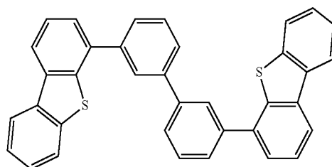
Compound 23
