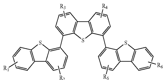
Compound 4G
