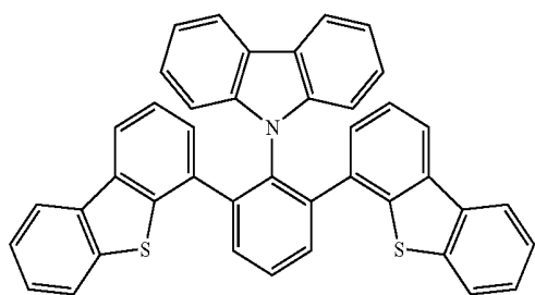
Compound 19
