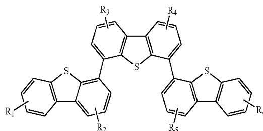
Compound 4G
