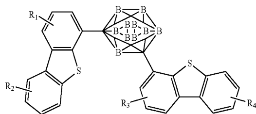
Compound 14G
