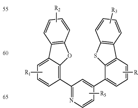
Compound 27G
