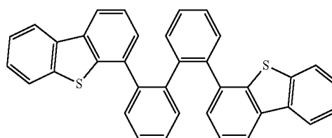
Compound 3
