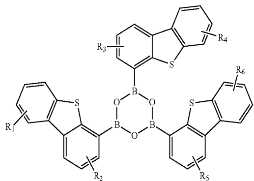
Compound 8G
