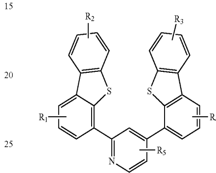
Compound 24G
