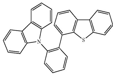
Compound 22
