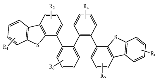
Compound 2G
