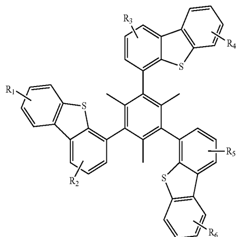
Compound 5G
