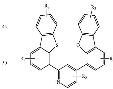
Compound 26G
