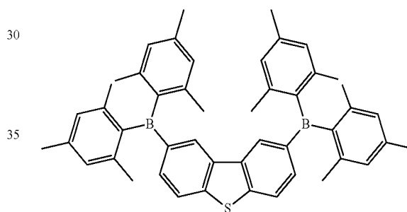
Compound 7
