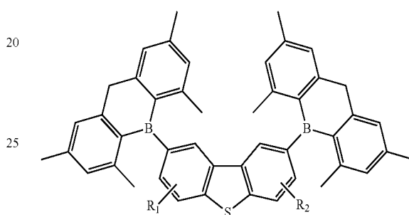
Compound 7G
