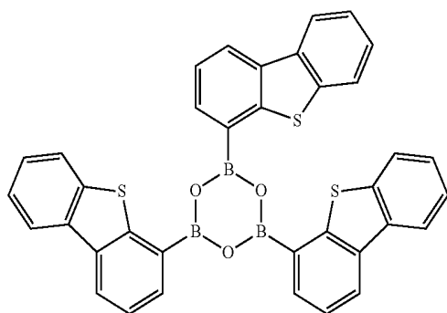
Compound 9
